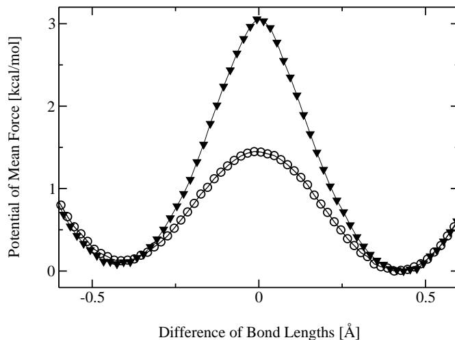
Figure 3.5: PMFs as a function of the difference of bond lengths involving the proton with the donor and acceptor oxygens in malonaldehyde. The \blacktriangledown curve is from classical EVB, while the \odot curve is from EVB/PIMD.
