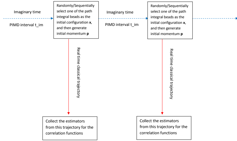
Figure 5.1: Flow chart for LSC-IVR.
